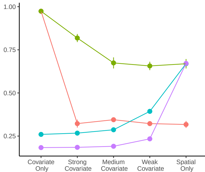
Coverage Rates
