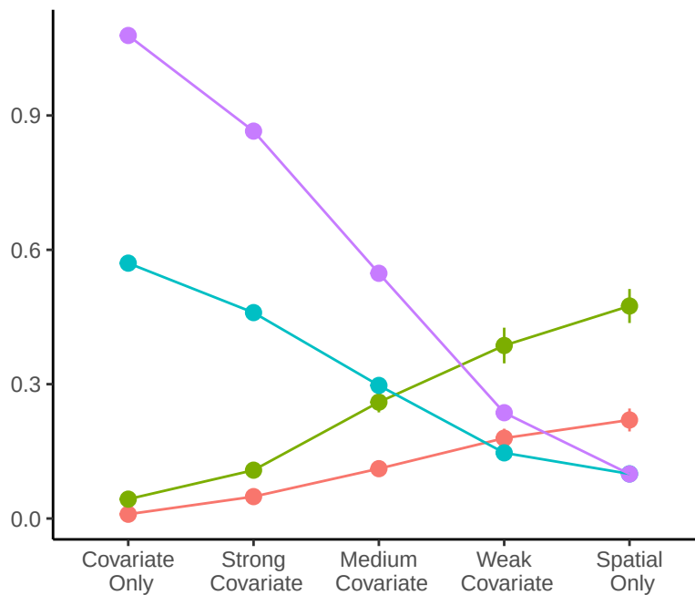
Interval Scores
