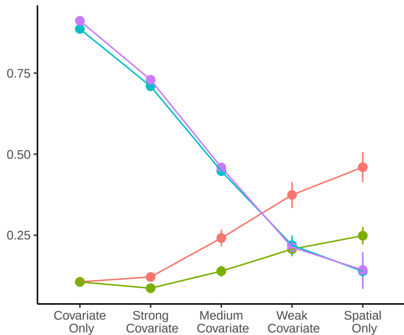
RMSE
